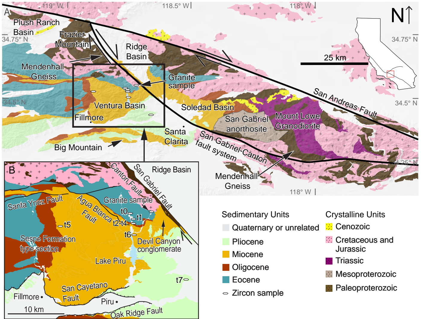
Figure 1: A) Geologic map of the eastern Ventura Basin (after Dibblee, 2010; Jennings, 2010; Jacobson et al., 2011). B) Inset map of the eastern Ventura Basin, showing sample locations t0-t7.
