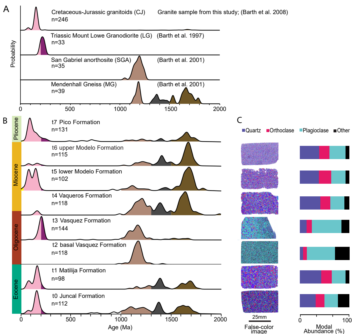
Figure 2: A) KDEs of zircon U-Pb dates from crystalline sources (parents). B) KDEs of DZ from eight Eocene-Pliocene samples (children). KDEs are not normalized and are constructed using a Gaussian kernel with a bandwidth of 20 Ma. C) Thin section false-color images of SAM data with abundant minerals labeled and bars plotting their modal abundances. The SAM and DZ data were analyzed from the same set of samples, but sample t7 was too disaggregated to make a thin section.
