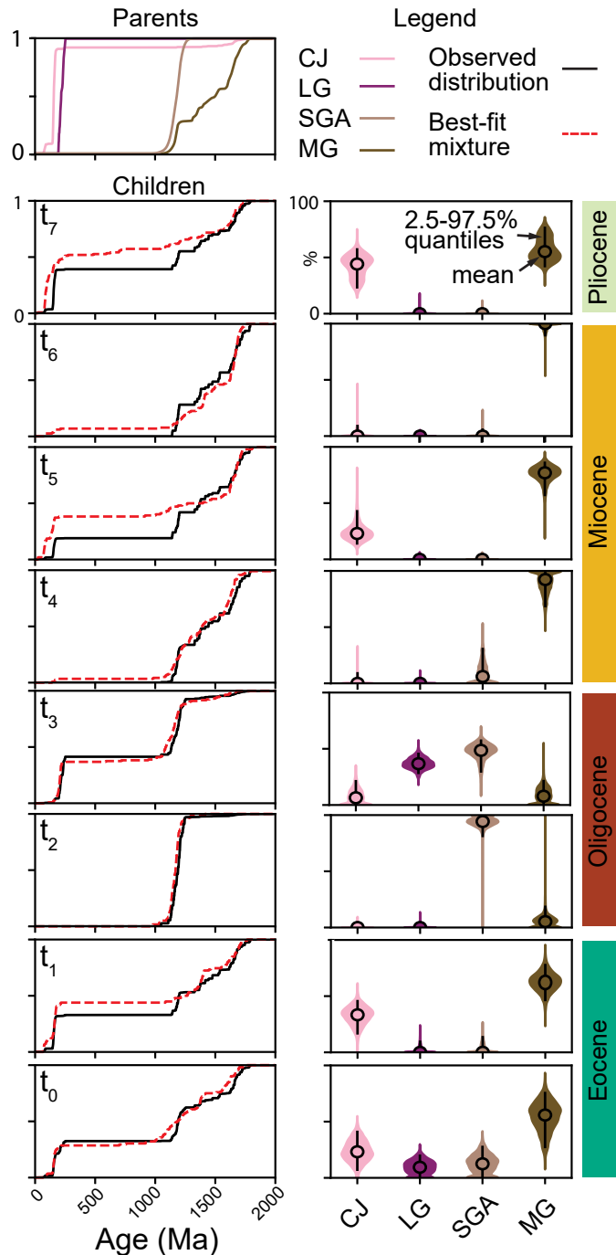
Figure 3: Left) Plots showing best-fit mixture-model results for each child sample using the Vmax comparison metric and the observed distribution. Right) Violin plots displaying range of uncertainty for each parent contribution from the resampling results.
