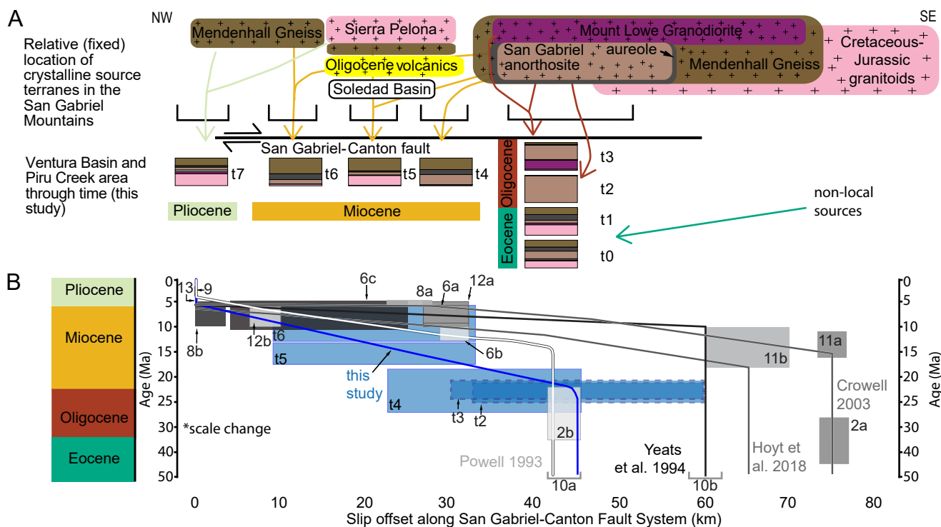
Figure 4: Compilation of the translational history of the Ventura Basin. A) Interpreted patterns of sediment routing and basin translation through time. Stacked bar charts show child sample DZ dates colored by parent age bins. B) Fault slip-offset diagram comparing our model that suggests 35–60 km of total slip to four published Ventura Basin reconstructions. Boxes represent fault slip uncertainty when reported and those with the same number in the label represent a different interpretation of the same piercing point (e.g. 2a, 2b, t2). Boxes constraining our model are colored blue and are labeled t2–t6 for consistency with the sample names. Boxes t2 and t3 are dashed because they represent interpretations with poor constraints.
